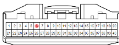
Vista frontal conector
