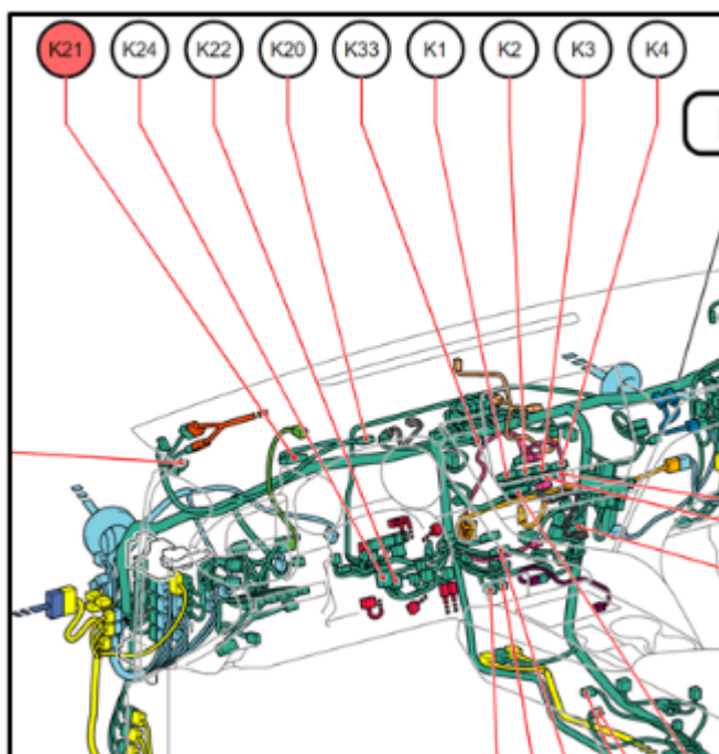
Vista frontal conector
